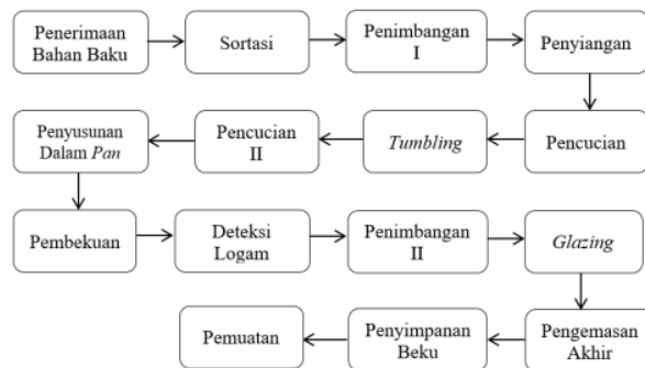
Gambar 2. Alur proses pengolahan gurita flower type
