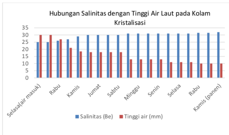
Gambar 6 . Grafik hubungan salinitas dan tinggi air pada kolam kristalisasi Figure 6. Graph of the relationship between salinity and water level in the crystallization pond
